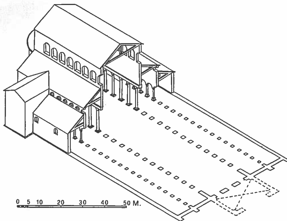
Fig. 3.3 S. Giovanni in Laterano. Isometric reconstruction. After CBCR.
