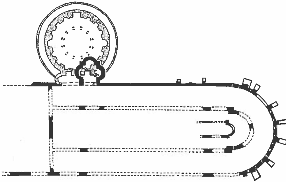
Fig. 3.44 Via Nomentana. Apse-ended basilica, mausoleum, and S. Costanza. After Mackie in Byzantium 67.
