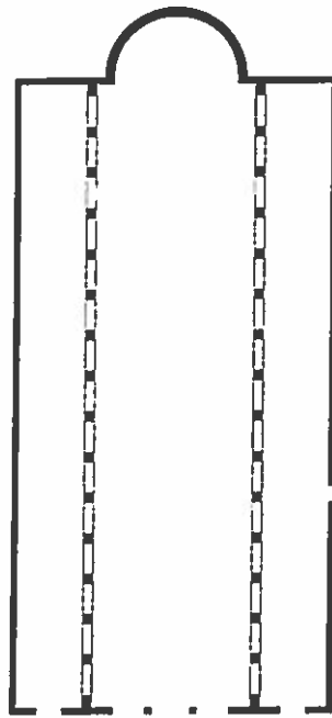
Fig. 3.25 Ostia, plan of the early Christian basilica. Courtesy Michael Heinzelmann.
