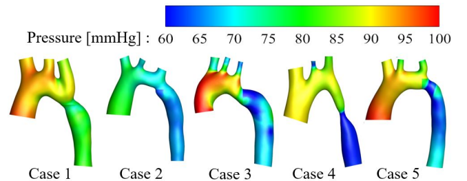
Fig. 2. Pressure distributions in five aortas with coarctation. Since the peak pressure occurs at different times in AAo and DAo, the pressure distributions of the areas proximal and distal to the coarctation were individually extracted at their respective peak times and juxtaposed for visualization.
